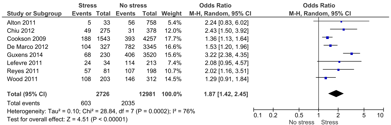
S6: Forest plot of the meta-analysis (dichotomous measures) on the association between any form of prenatal maternal psychological stress and wheezing in childhood.
