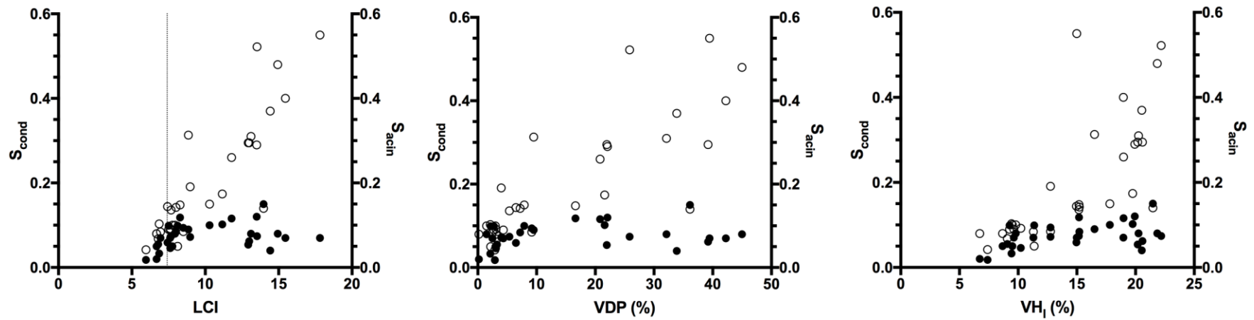
Figure S5: Scatterplots of S_{acin} (open circles, right Y axis) and S_{cond} (closed circles, left Y axis) against; LCI (dashed line indicates the upper limit of normal), VDP and VH_I . S_{cond} consistently demonstrates a plateau effect with increased levels of disease severity, without evidence of statistical correlation. S_{acin} however demonstrates significant correlations with LCI ( r=0.86 ), VDP ( r=0.84 ) and VH_I ( r=0.82 ).
