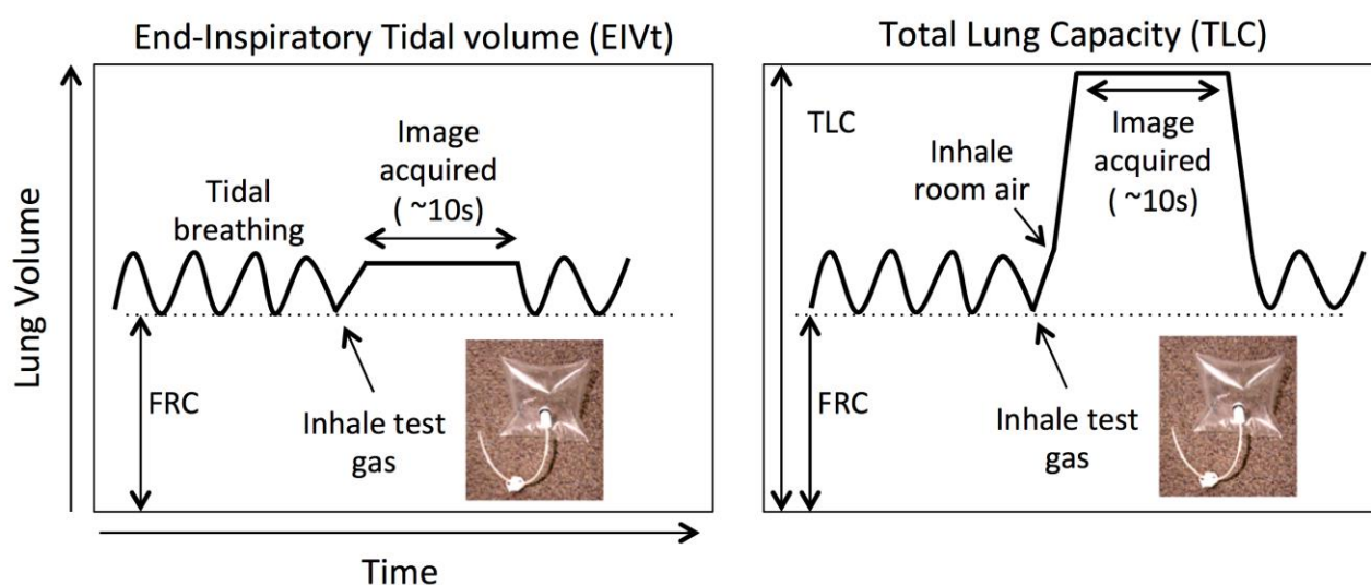
Figure S1: Schematic detailing the breathing sequence performed for both EIVt and TLC ventilation imaging highlighting the difference in the lung volumes for the two MR image acquisitions.
