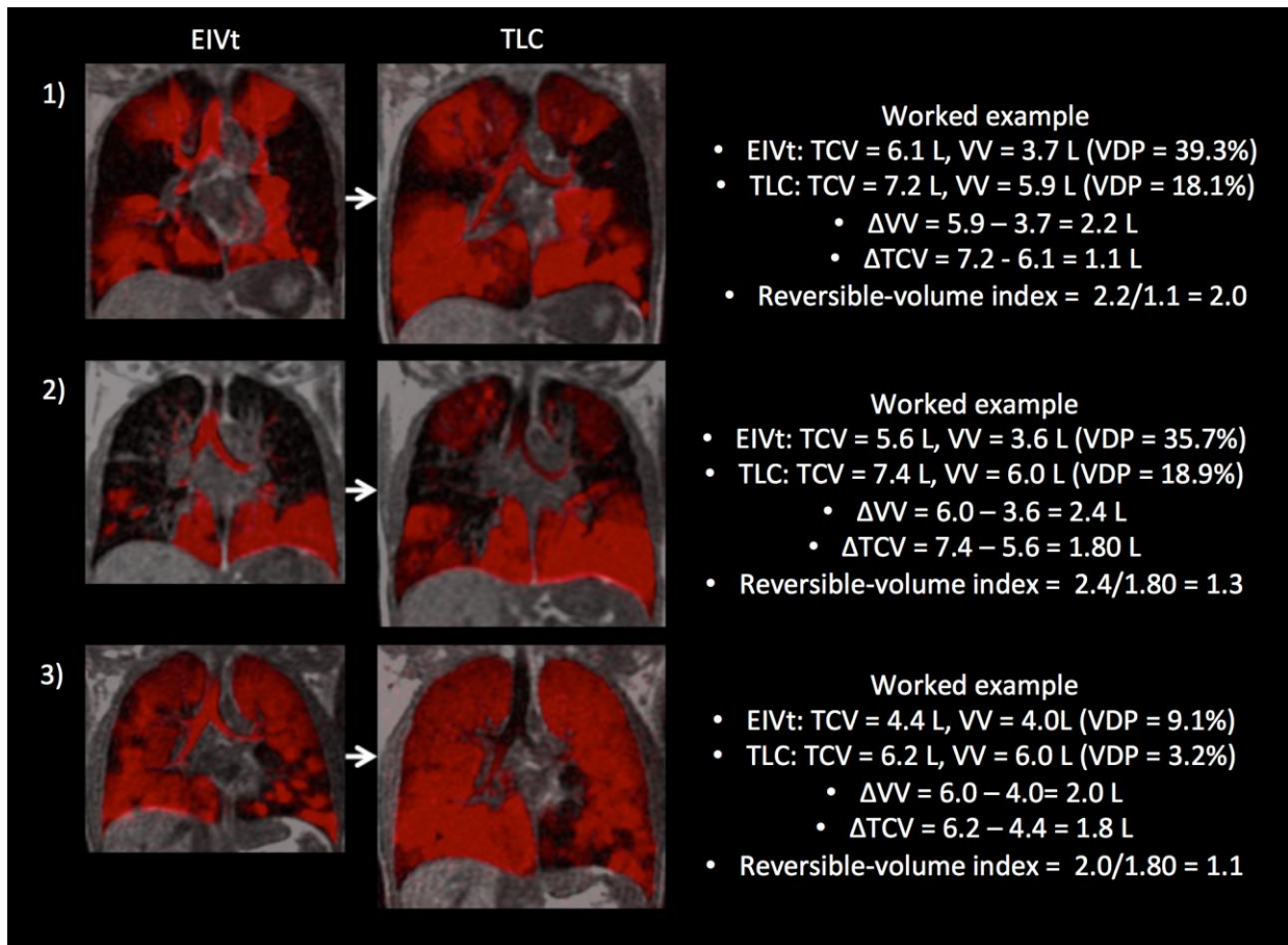
Figure S3: Worked reversible-volume index examples from different patients (1-3) within the study. Representative EIVt and TLC ventilation image slices (red) are overlaid onto the ^1\text{H} MRI acquired during the same breath-hold (grey). The ventilated volume (VV) is calculated from the segmentation of the ^3\text{He} ventilation image and the thoracic cavity volume (TCV) is calculated from the segmentation of the ^1\text{H} image. Both the TCV and VV are measured in litres (L).
