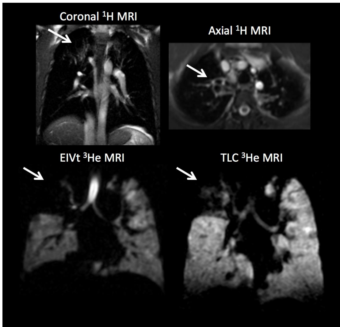
Figure S7: EIVt and TLC ^3\text{He} comparison for a patient with CF and representative ^1\text{H} anatomical MR imaging demonstrating bronchiectasis. At EIVt this patient has
