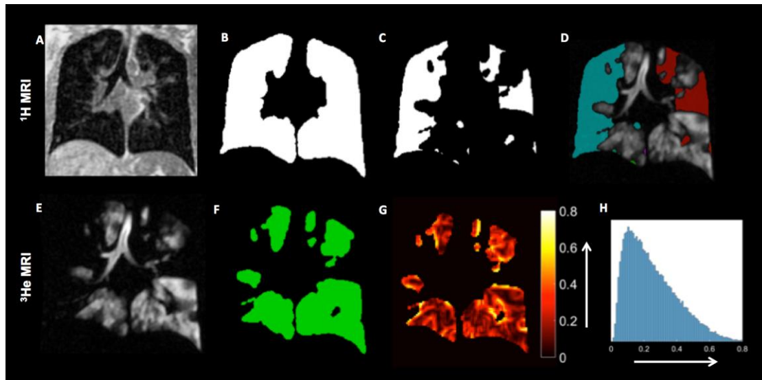
Figure S2: Workflow of ventilation image analysis from one patient. The ^1\text{H} anatomical image (image A) and the ^3\text{He} ventilation image (E) are segmented to create a thoracic cavity mask (B) and a ventilation mask (F). Ventilation defect percentage is calculated from the resulting mask volumes. The ventilation defect mask (C) is created as the inverse of the ventilation mask within the thoracic cavity mask (B) and is used to assess the number and volume of contiguous ventilation defects (D). Individual contiguous ventilation defects are shown in different colours in D. The ventilation mask (F) is used to define the area over which the local coefficient of variation is calculated from a 3*3 moving window centred on
