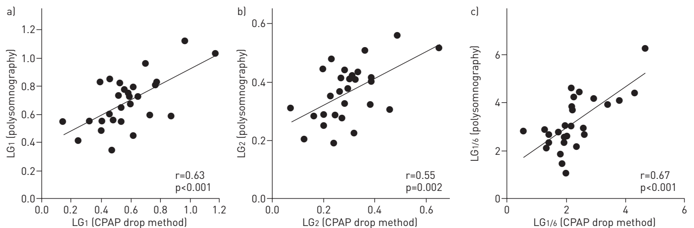
FIGURE 4 Comparison of our method and the continuous positive airway pressure (CPAP) drop method for measuring loop gain. Agreement was observed across a range of frequencies including a) “mid-frequency” ( 1\text{ cycle}\cdot\text{min}^{-1} ( LG_1 )), b) “high frequency” ( LG_2 ) and c) “low frequency” ( LG_1/6 ; 6-min period). Note that loop gain (the chemical drive response to a reduction in ventilation) is a function of the frequency (e.g. timing) of the disturbance in ventilation.
