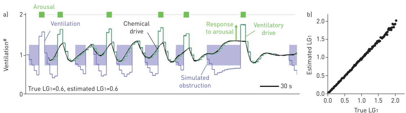
FIGURE 2 Mathematical model validation. a) Example simulation showing that loop gain is accurately recovered from ventilation in a model of obstructive sleep apnoea (loop gain, LG_1 is the response to a 1\text{-cycle}\cdot\text{min}^{-1} disturbance). Shaded regions denote periods of obstruction. The estimated chemical drive (solid smooth black line) is precisely superimposed on true chemical drive (dashed black line is not visible due to near-perfect overlap); likewise, estimated ventilatory drive (green staircased line) is closely overlaid upon the observed ventilation (blue staircase line) in the absence of obstruction. b) Group simulation data show that the method accurately reveals the true loop gain given to the model. Model parameters: delay 12 s, time constant 12.5 s and response to arousal 0.4 (40% eupnoeic ventilation). Obstructive events were imposed by halving the controller gain (doubling resistance) for three or more breaths at random times in a graduated manner. Arousals were imposed for two breaths at the termination of 80% of obstructive events and on 1% of unobstructed breaths. #: normalised such that 1=eupnoea.
