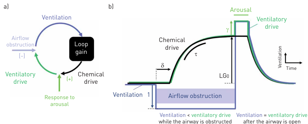
FIGURE 1 Mathematical basis of the method. a) Schematic of the feedback loop controlling ventilation showing the influence of arousal and airflow obstruction. Ventilatory drive is the sum of chemical drive and the response to arousal ( \gamma ) (equation 1 in the main text). Airflow obstruction provides a disturbance that reduces ventilation from the intended level (i.e. ventilatory drive). In response, chemical drive rises as determined by the chemical control system (loop gain). b) Time course of chemical drive during a step reduction in ventilation (e.g. obstructive hypopnoea). The rise in chemical drive is governed by and the parameters that determine its gain ( LG_0 ), time constant ( \tau ) and delay ( \delta ) (equation 2 in the main text); these system characteristics are revealed in the time course of ventilation when the airway is reopened.
