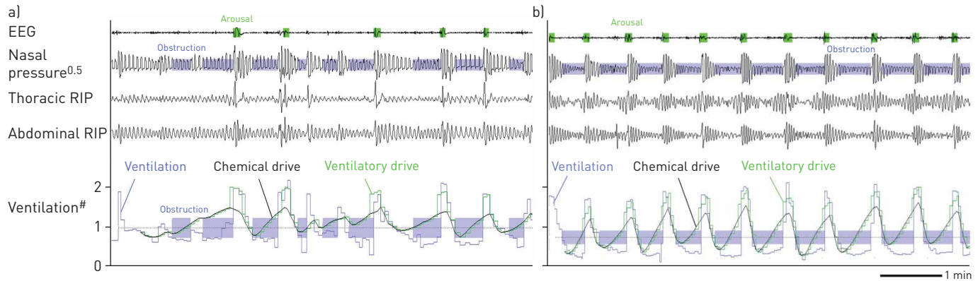
FIGURE 3 Estimating loop gain using diagnostic polysomnography. Example traces illustrate epochs with a) relatively low loop gain (response to a 1\text{-cycle}\cdot\text{min}^{-1} disturbance ( LG_1 )=0.6) and b) relatively high loop gain ( LG_1 =1.1). Note that ventilatory drive (chemical drive + response to arousal) closely fits ventilation during periods of unobstructed airflow. Loop gain determines the increase in chemical drive in response to the reduction in ventilation. EEG: electroencephalogram; RIP: respiratory inductance plethysmography. #: normalised.
