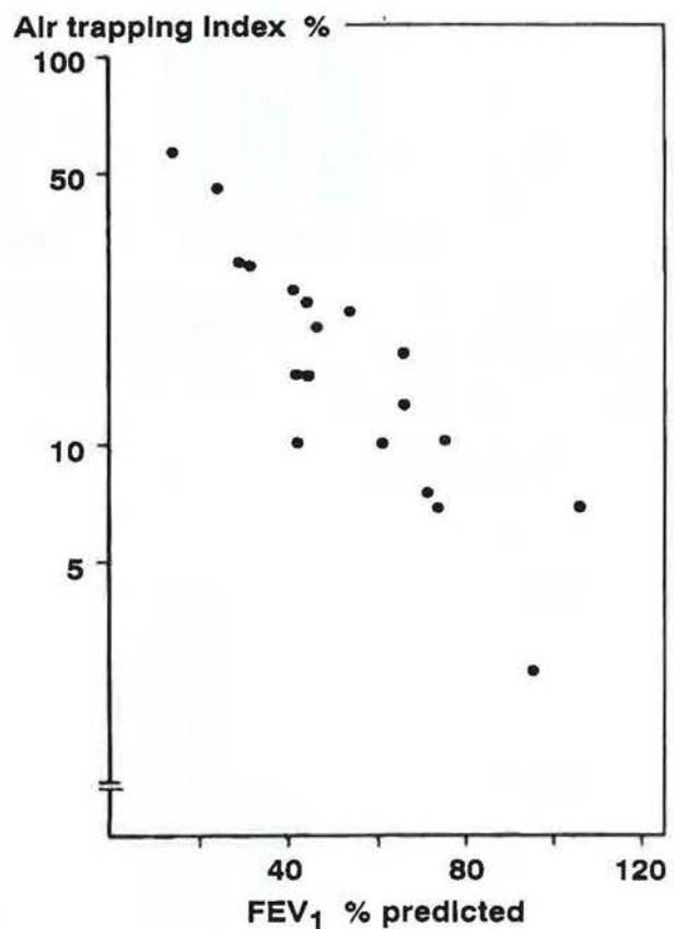
Fig. 1. - Correlation between air trapping (AT) index and baseline FEV 1 (% predicted) in 20 adult CF patients. Log expression of AT-index is used. R_{yx} = -0.83 ; p=0.0008 . CF: cystic fibrosis; FEV 1 : forced expiratory volume in one second.
