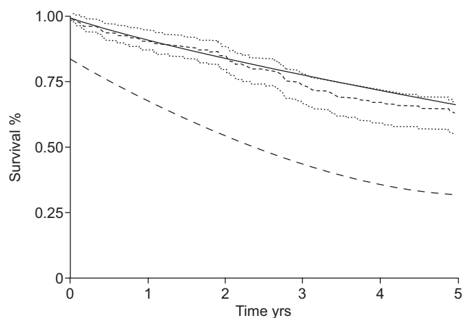
FIGURE 3. Observed (-----; 95% confidence interval: ..... ) versus predicted survival using the Pulmonary Hypertension Connection (—) and National Institutes of Health (---) equations in patients with idiopathic, familial and anorexigen-associated pulmonary arterial hypertension.
