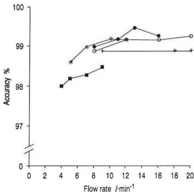
Fig. 3. — Accuracy of dry gas meter A at continuous and resting sinusoidal flows. % accuracy = (gas meter volume/Collins gasometer volume) \times 100 . —+—: continuous flows; —■—: 0.4 l at 8–20 br·min -1 ; —*—: 0.6 l at 8–20 br·min -1 ; —●—: 0.8 l at 8–20 br·min -1 ; —○—: 1.0 l at 8–20 br·min -1 .
