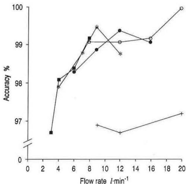
Fig. 4. — Accuracy of dry gas meter B at continuous and resting sinusoidal flows. % accuracy = (gas meter volume/Collins gasometer volume) \times 100 . For key to symbols see legend to figure 3.
