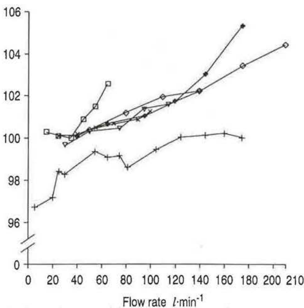
Fig. 2. - Accuracy of dry gas meter B at continuous and exercising sinusoidal flows. % accuracy=(gas meter volume/Collins gasometer volume) × 100. For key to symbols see legend to figure 1.
