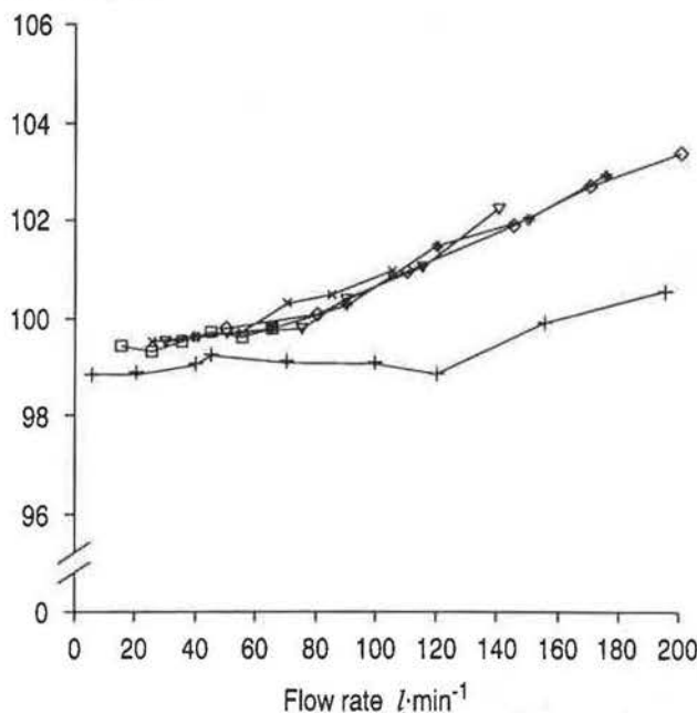
Fig. 1. - Accuracy of dry gas meter A at continuous and exercising sinusoidal flows. % accuracy=(gas meter volume/Collins gasometer volume) × 100. —+— : continuous flows; —□— : 1.0 l at 15–65 br·min -1 ; —*— : 1.5 l at 15–65 br·min -1 ; —▽— : 2.1 l at 15–65 br·min -1 ; —#— : 2.6 l at 15–65 br·min -1 ; —◇— : 3.1 l at 15–65 br·min -1 .
